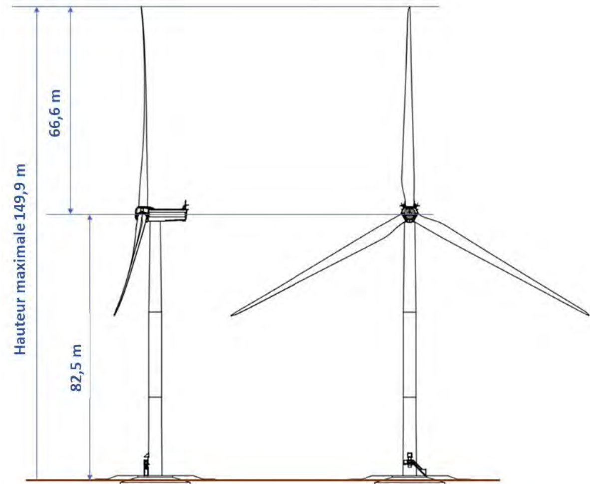
FIGURE 12 - EOLIEENNE NORDEX
